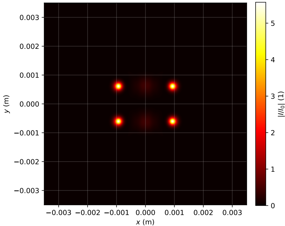
Intensity profile I(x, y, z = 1.433)/I_0 , P_{in}=5.0P_{cr} , artificial time
